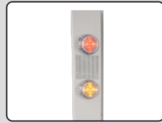
SOLAR GUIDE POST Ht.-1250mm Flasher Dia.-80mm, 18 nos. LEDs
