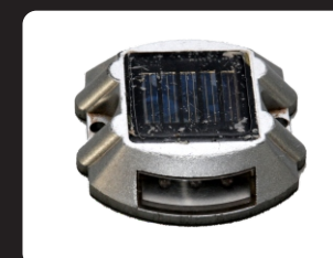
SOLAR ROAD STUD (SRS-01) 110x93x20mm Flat Base
