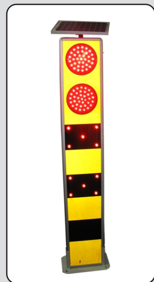
TWIN SOLAR WARNING BOLLARD Ht.-1600mm, 02x200mm Dia. Blinkers
