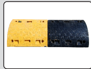
RUBBER SPEED BUMP (75mm) 415x500x75mm
